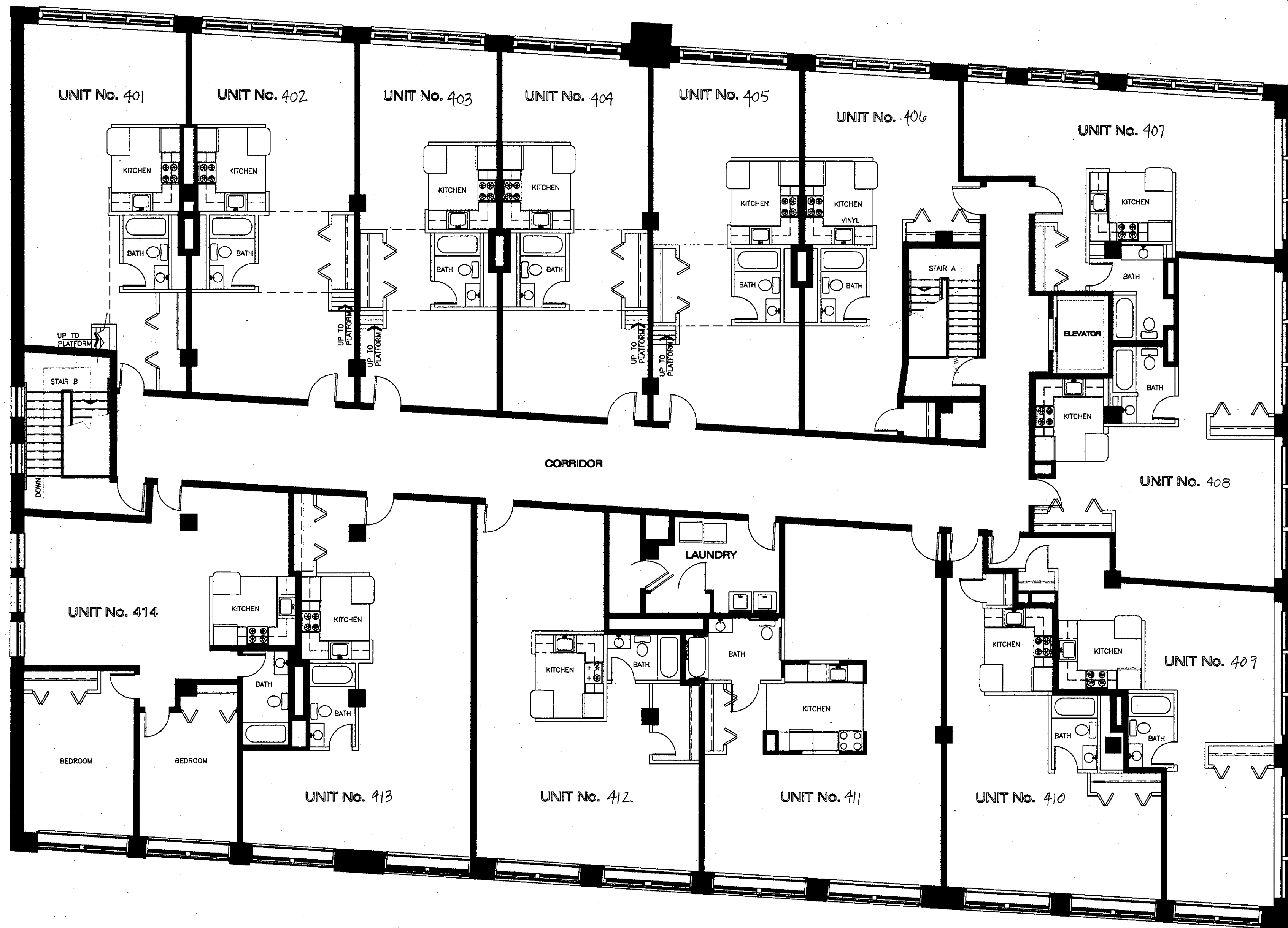
FOURTH FLOOR PLAN
