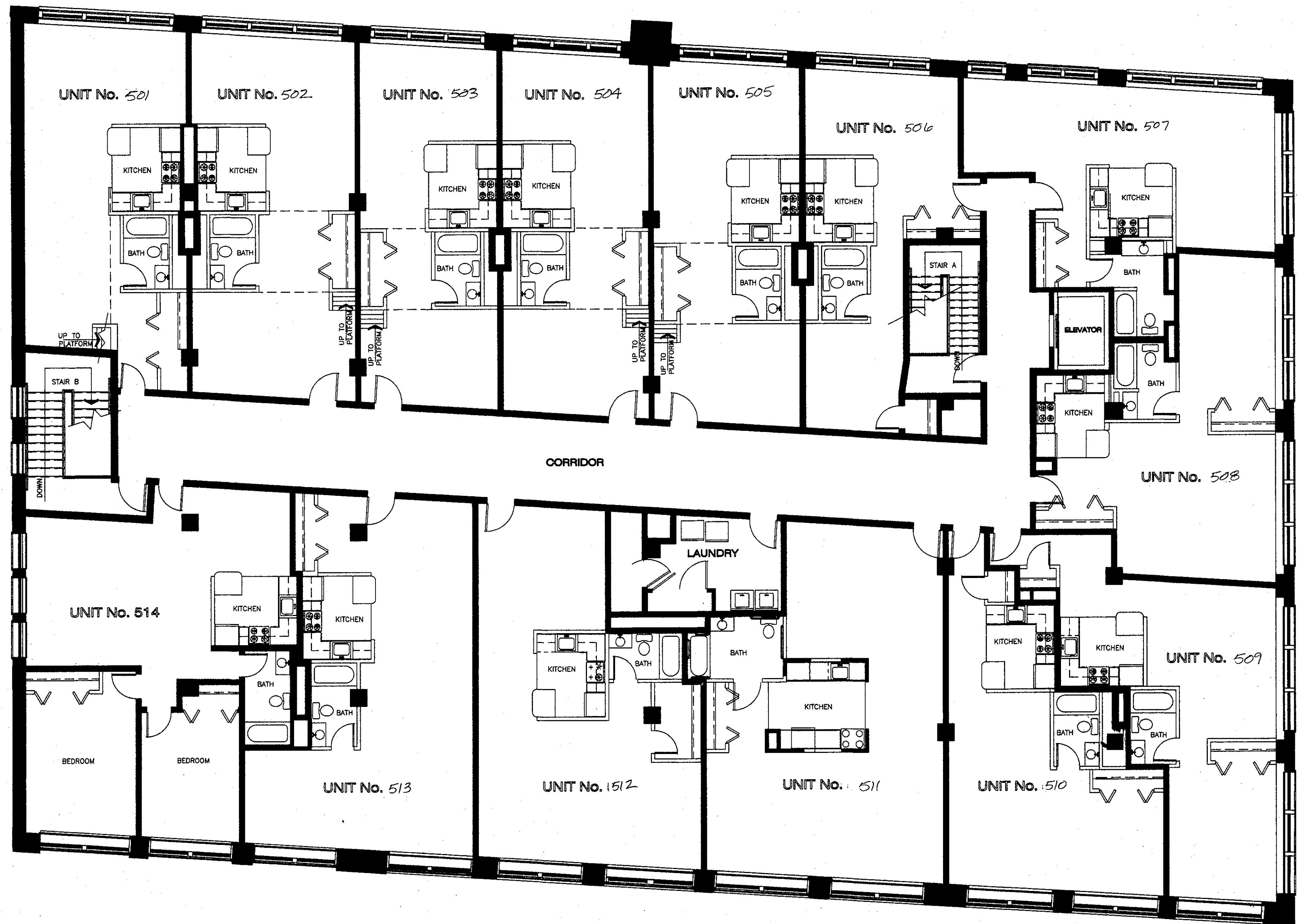
FIFTH FLOOR PLAN
